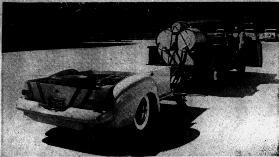
DELUXE SKID TRAILER — Designed to be towed behind a light truck is this "skid trailer" developed by General Motors Proving Ground staffers for checking the coefficient of friction or
