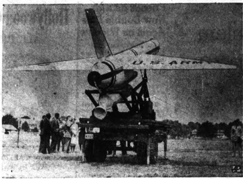
SEEKS INFORMATION—A scout drone, the U.S. Army's latest device for gathering data behind enemy lines, is displayed on its mobile launching platform at Ft. Myer, Va. The instrument-packed, pilotless craft is 36 feet long and has a 24-foot wing span.
