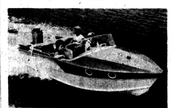
RAISED DECK — An outboard cruiser maintains hull strength by unbroken forward deck beams, obtaining headroom by subtly rising sheer.
