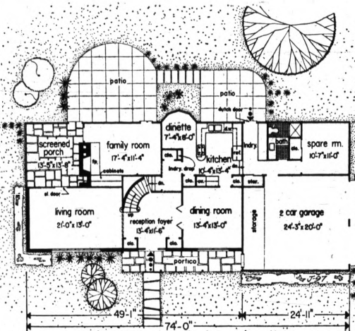
FASHIONABLE ELEGANCE —This subdued and tasteful home has four large bedrooms, plus a spare bedroom, among its nine full rooms. The floor plan is straightforward within simple and direct framing and the exterior shows the innate beauty of simplicity. The architect is Samuel Paul.
