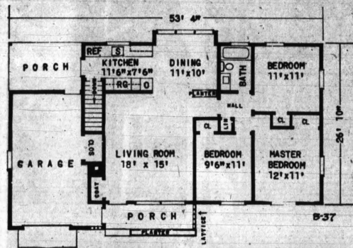
FLOOR PLAN —Efficient and original use of space make this small ranch an interesting home. Note especially the well-placed basement stairs, right next to the service entrance.
