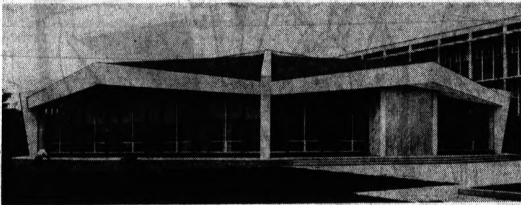
UNUSUAL DESIGN — The new County Courthouse auditorium breaks away from conventional rectangular architecture. Most of the exterior of the six-sided building is of brick and glass. The doors are of aluminum. Behind the auditorium to the right can be seen part of the courthouse wing with a connecting corridor.
