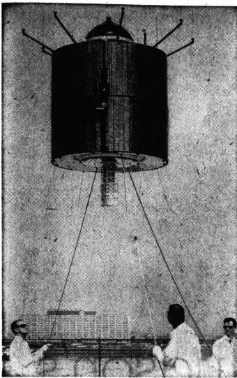
GOING FOR SPIN —The newest applications technology satellite (ATS) hangs from a huge crane as it is put through an antenna pattern test by engineers at Hughes Aircraft Co., El Segundo, Calif., which builds the satellites for NASA. This ATS is slated for a Nov. 7 launch from Cape Kennedy to take color photos of the Western Hemisphere's weather conditions and to conduct communications and navigation experiments.
