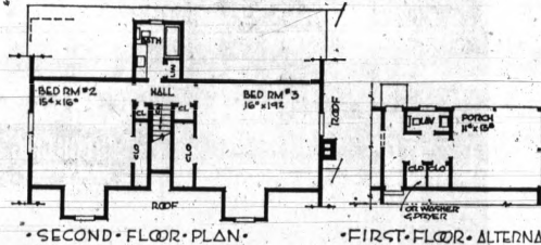
SECOND FLOOR PLAN • FIRST FLOOR ALTERNATE
