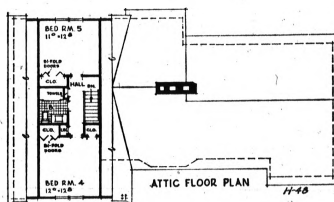
FLOOR PLANS: Expandable features make this home suitable for family requiring from two to five bedrooms. Also, note long sweep from living room through dining room and from Harvest Room through kitchen.
