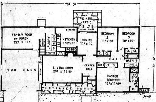
FLOOR PLANS —The living area covers 1,320 square feet plus an additional 325 square feet for the laundry and porch-family room. The basement lies under the living, dining and sleeping areas. Note the separation of living, sleeping and utility centers.
