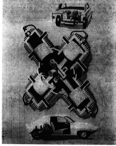
NEW CAR IDEA — Drawings show the "X-4," a new three-passenger car idea with a radically new type of engine said to be under development by Pontiac Motor Division. The design appeared in the April edition of Popular Science Monthly magazine. Top and bottom drawings show how the engine is mounted in the car. At center is the new radial engine, with opposing pistons sharing a one-piece connecting rod. The back-and-forth motion of the connecting rod is transmitted into rotary motion by crankpins which slide back and forth in slots in the connecting rods.
