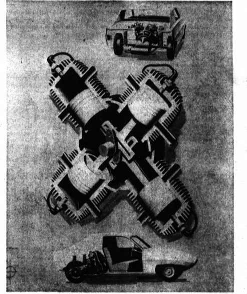
NEW CAR IDEA — Drawings show the "X-4," a new three-passenger car idea with a radically new type of engine said to be under development by Pontiac Motor Division. The design appeared in the April edition of Popular Science Monthly magazine. Top and bottom drawings show how the engine is mounted in the car. At center is the new radial engine, with opposing pistons sharing a one-piece connecting rod. The back-and-forth motion of the connecting rod is transmitted into rotary motion by crankpins which slide back and forth in slots in the connecting rods.
