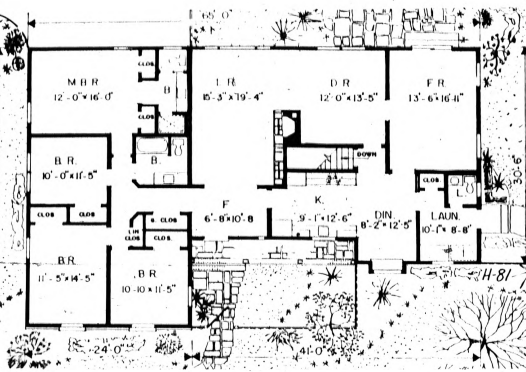
FLOOR PLANS: A good traffic pattern here. Note, for example, how the family room can be entered from the living room-dining room combination, from the kitchen-dinette, from the side entrance and from the rear patio.
