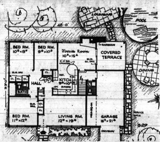
FLOOR PLAN — There are no cost-adding extra corners or recesses in the exterior walls. Note central location of the kitchen and convenient positioning of basement stairs and lavatory.
