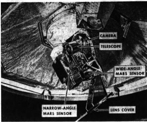
TO SNAP PICTURES — This is the heart of the photographic equipment on Mariner 4 which will attempt to take close-up pictures of the planet Mars tomorrow night. If all goes well, 21 photographs will be taken and relayed back to earth.
