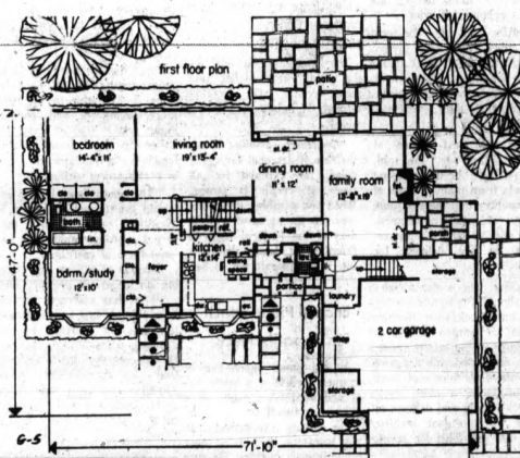
FLOOR PLANS: The traffic pattern, fundamentally sound for the rooms on the left side of the house, takes on additional
