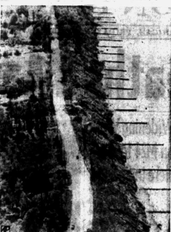
HIGHWAY THREATENED —Airflow of U. S. 12 near St. Joseph, comes close to edge of bluff overlooking shores of Lake Michigan. Note particularly in lower right-hand corner. Cracks can be seen in face of bluff where highway comes near drop. Erosion of bluff in recent years has forced abandonment of several lake-front homes.
