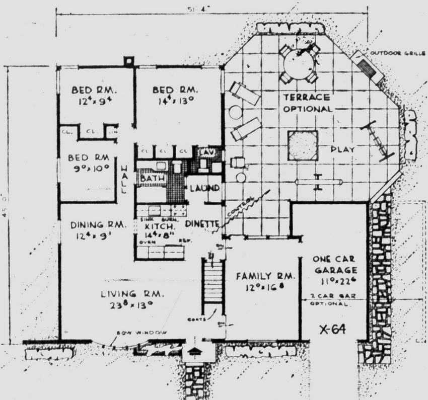
FLOOR PLAN — Family room and garage provide X-64 with a wide front wall, even though main section of the house is a rectangle with narrow end at front. Central location of kitchen makes it easy for housewife to reach any section of the home.
