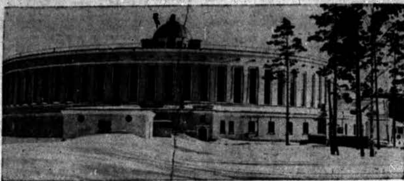
REDS BUILD BIG SYNCHROCYCLOTRON —Moscow reports erection of the world's largest synchrocyclotron. The giant machine, designed for studying the atomic nucleus, was developed by the U. S. S. R. Academy of Sciences. The circular building, above, is the central block where the synchrocyclotron is installed. Its circular magnet weighs 36,000 tons and has a diameter of nearly 200 feet. Photo and caption material from Soviet sources.
