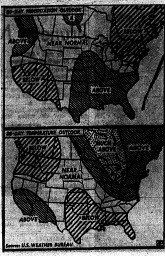
THIRTY-DAY FORECAST — These maps, based on those supplied by the U.S. Weather Bureau, forecast the expected precipitation and temperature for the next 30 days. Temperature for the Pontiac area will be above average but the precipitation will be normal.
