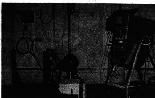
HELMET TEST — The retention system of motorcycle helmets manufacturers want to place on the market is tested at firms like the Detroit Testing Laboratory, Inc., (above) of Oak Park. The helmet is mounted on a head form and a weight is dropped on it. Instruments in the head form measure the force transmitted to it. The transmitted force is measured on the oscilloscope (right).
