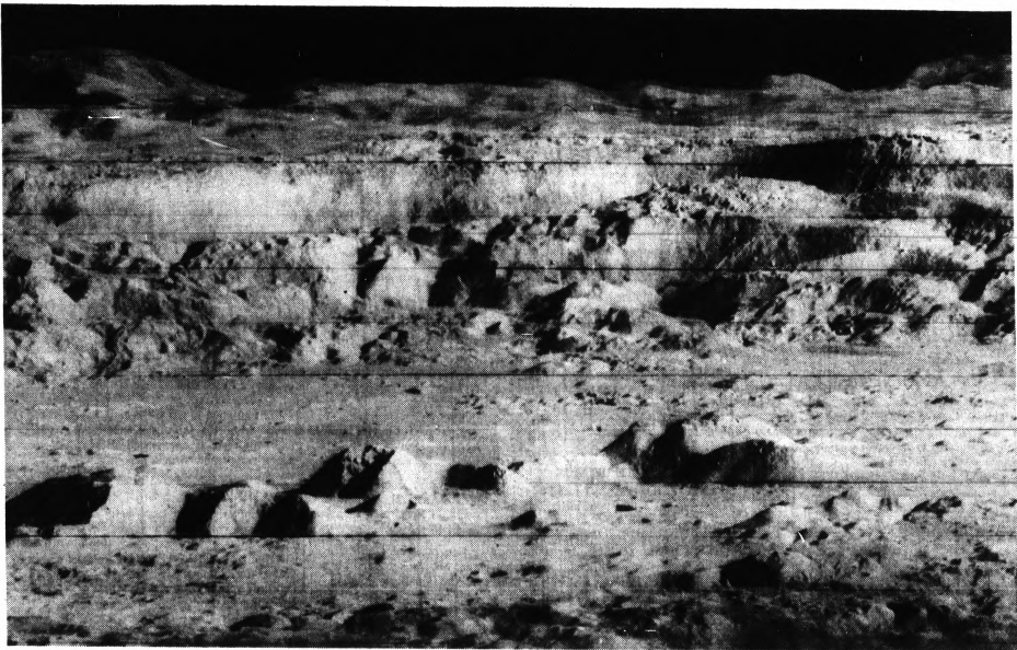
MOON PHOTO RELEASED — This close-up photograph of the moon crater Copernicus, a prominent feature on the lunar surface, was released today in Washington. It was taken Nov. 23 by Lunar Orbiter II. The view looks down the floor area 1,000 feet high with slopes up to 30
