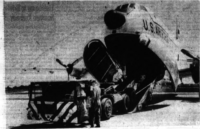
LOADED AT SELFIDGE — A huge, six-ton missile transporter developed by General Motors Truck and Coach Division is undergoing inspection by the U. S. Air Force in Seattle, Wash., today. It is designed to haul Minuteman ICBMs to underground launching sites. The unusual vehicle is shown being loaded into the cargo body of a C-124 "Globemaster" yesterday at Selfridge Field for its cross-country hop. (Story on page 2.)
