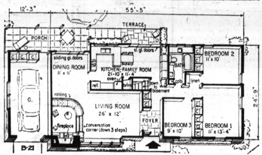
FLOOR PLAN — House has few variations from basic rectangular shape, which makes for economy in construction. Entrance foyer insures good circulation pattern.
