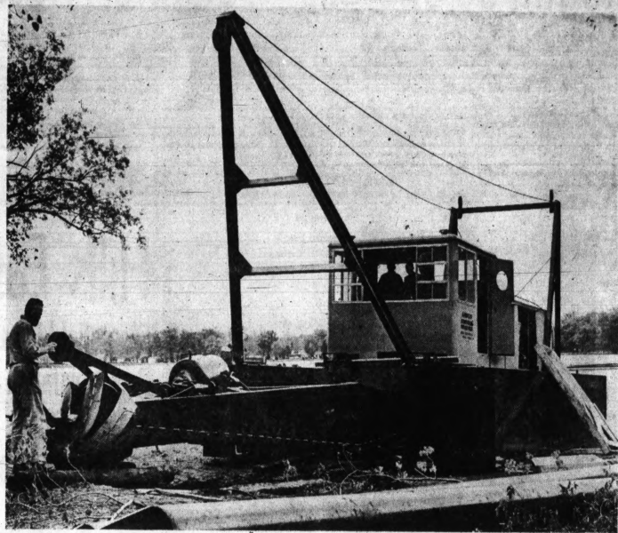
GIANT DREDGE —A workman stands in front of the business end of a 45-ton dredge that will begin operations next week to clean and deepen Long Lake in Commerce Township. The machine, which will be used to restore the 3-foot deep lake to a depth of more than 10 feet, is owned by the Waterways and
