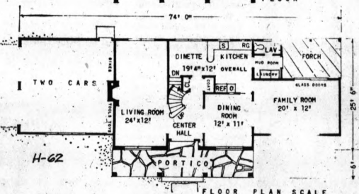
FLOOR PLANS — King-size family can be accommodated in this four-bedroom Colonial, with a well-designed service area at the rear of the house and a large family room for informality.
