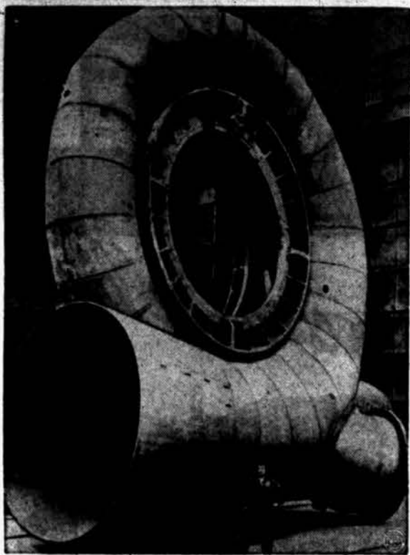
BRITAIN'S INDUSTRY ROOMS — This huge, horn-like spiral casing in London, England, will house plenty when filled with a 73,000-horsepower water turbine and shipped to Portugal. The 35-foot-high, 66-ton casing dwarfs the man at bottom of photo. Great Britain is in the midst of a new industrial export boom.
