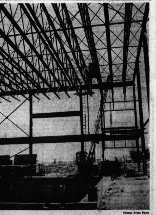
THE UPWARD LOOK — At Michigan State University Oakland this steel structure is rising over what in the fall will be a 102-by-97-foot swimming pool — part of the 1.5-million-dollar Intramural Sports and Recreation Building.
