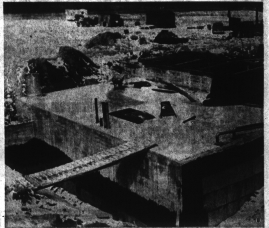
AT HALF-WAY MARK —Construction is 50 per cent complete at the two Nike bases in Oakland County. Shown above is a partially completed missile-launching pit at the site near Squirrel and Featherstone Rds., in Avon Township, north of Auburn Heights. Another base is planned for Commerce Township, near Milford.
