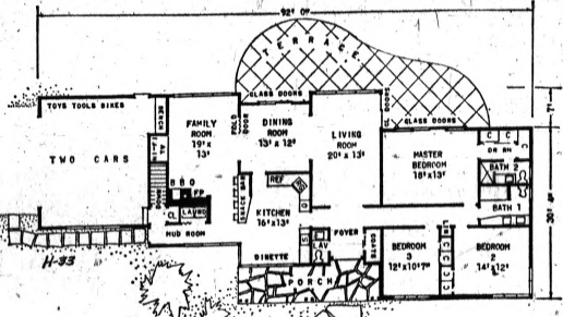
FLOOR PLAN: An H-shape layout, with the family and living rooms forming the vertical lines and the dining room forming
