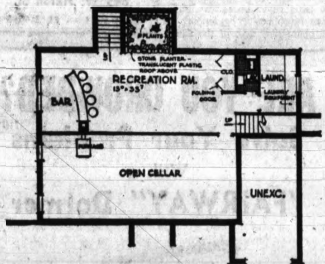
BASMENT PLAN —Recessed garden, underneath translucent skylight, gives recreation room a unique focal point.
