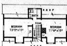
SECOND FLOOR PLAN CORNER BATH VERSION
