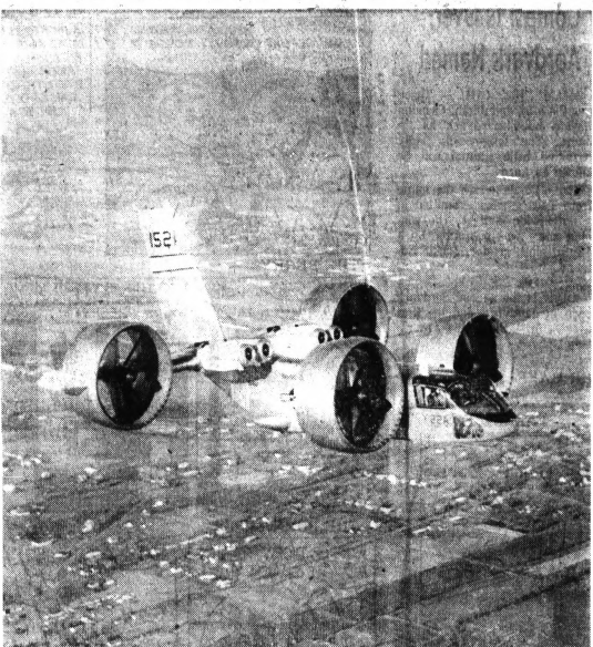
CRUISING ALONG — The X22A vertical takeoff and landing aircraft, built by Textron's Bell Aerosystems Co., soars over the countryside near Niagara Falls, N.Y., on its
