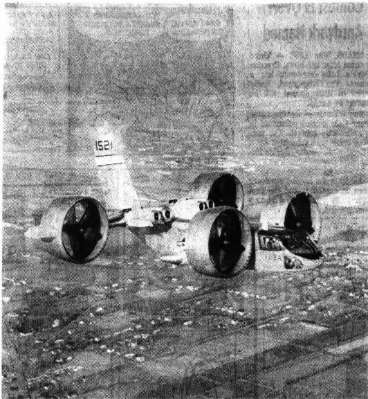
CRUISING ALONG — The X22A vertical takeoff and landing airplane, built by Textron's Bell Aerosystems Co., soars over the countryside near Niagara Falls, N.Y., on its
