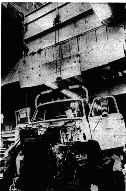
The Cab Drops From Above To The Frame
