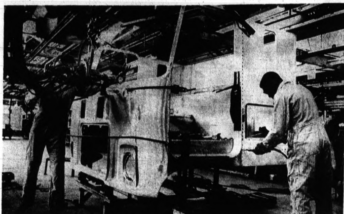
Stamped Parts Are Assembled And Welded To Form Astro 95 Cab
