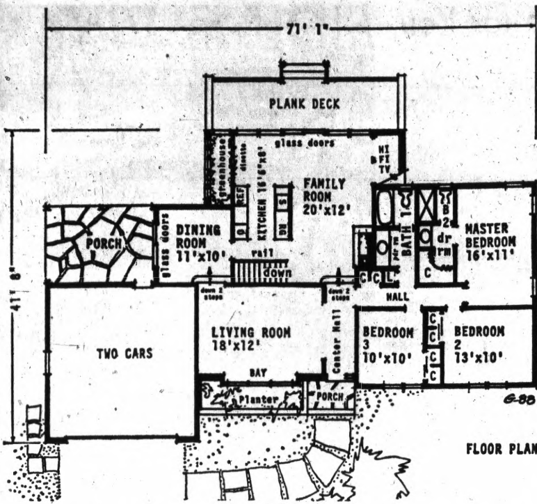
FLOOR PLANS: Informal living is stressed here, with the family room, dining room and kitchen two steps down from the rest of the house and tied in with a plank outdoor deck at the rear and a slate-floored porch at the side of the dining room.
