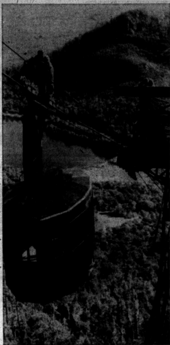
PLENTY OF FRESH AIR ON JOB — Don Johnson, of Littleton, N. H., stands atop the carriage of an ascending car of the Cannon Mountain Aerial Tramway as he makes daily inspection of the mile-long track cable. The state-owned tramway, used by skiers in winter and tourists in summer, rises over 2,000 vertical feet to 4,017-foot summit. Tilt's Echo Lake in the valley below.
