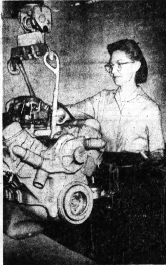
WIRED FOR POWER — Engine plant worker Mrs. Arlene Brown of 2341 Edinburgh St. installs spark plug wires on completed V-8 engines, which then go on to test stations for an operability check. Some of the engines will be shipped to six other points in the United States for Pontiac assembly.
