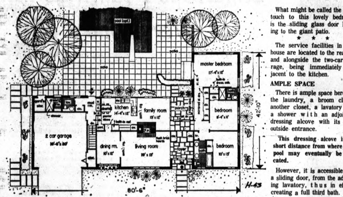
FLOOR PLANS — Everything in this house is designed to provide its occupants with an opportunity to live graciously and to entertain in style, either indoors or outdoors.
