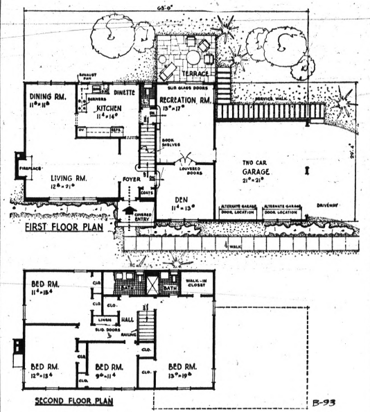
FLOOR PLANS - The clear separation of formal, informal and work areas of this house makes it extremely livable. Note also the abundance of closet space upstairs, especially the extra hall closet and the two walk-in closets in the master bedroom. House has a full basement.
