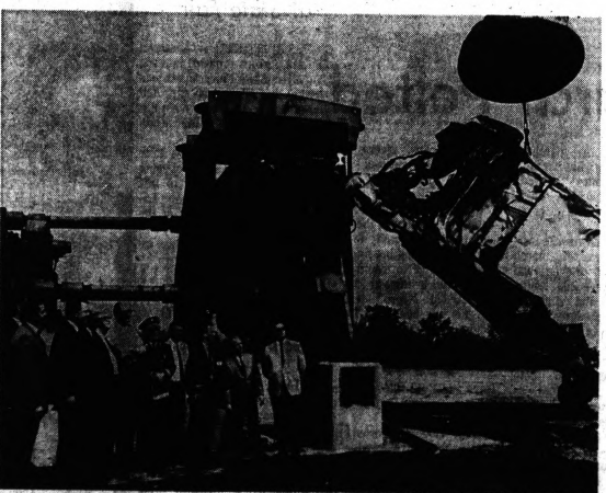
RIPPING DEMONSTRATION — City officials get a sneak preview of a new machine, the Rhino-autoripper, being fed its first meal. The machine, installed at Sam Allen & Sons, Inc., on Pontiac's North Side, transforms junk cars into foundry-usable chunks of metal.
