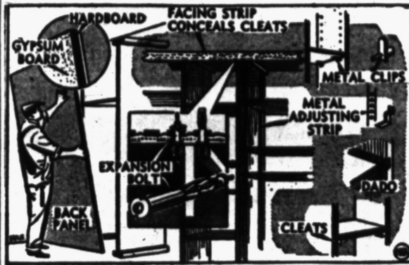
SPACE SOLVERS—Illustrated above are a thin-wall partition, left, methods of fastening ceiling cleats, center, and of hanging shelves.
