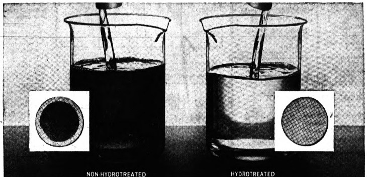
See the difference Shell's Hydro-desulphurization process can make in heating oil quality. Both oil samples were laboratory "aged" under identical conditions—250° F. for 16 hours. Non-hydrotreated oil (left) formed the dark sediment shown on sulphur filter pad, inset. Sediment can lead to trouble in your burner. But Shell hydrotreated oil (right) formed only the barest trace of sediment.
