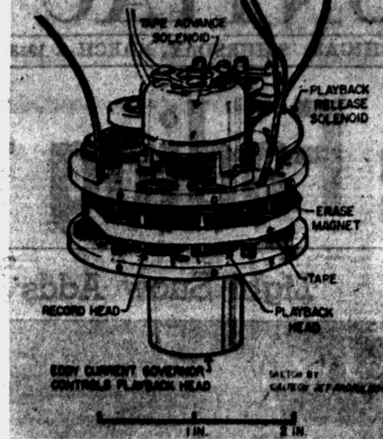
TAPE RECORDER ABOARD — This is a sketch of a magnetic tape recorder installed in Explorer II. It is designed to broadcast information to ground tracking stations, and is a new device not included in Explorer I.
