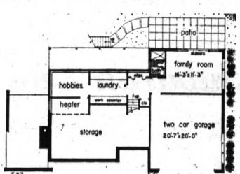
FLOOR PLANS — Mid-level area includes living room and foyer plus covered porch (which could be added later). Living and sleeping levels contain 1,388 square feet; lower level contains 1,023 square feet including garage. Porch adds 240 square feet and deck 174 square feet.
