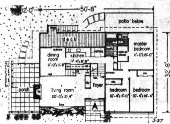
DRAMATIC B-LEVEL — With the silhouette of a handsome split-level, this bi-level model features a living room on the same entrance level as the foyer. It contains three bedrooms, 2½ baths in less than 1,600 square feet of living area, has a covered porch, covered rear deck, and patio.
