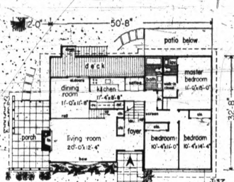
DRAMATIC BILEVEL — With the silhouette of a handsome split-level, this b-level model features a living room on the same entrance level as the foyer. It contains three bedrooms, 2½ baths in less than 1,400 square feet of living area; has a covered porch, covered rear deck, and patio.
