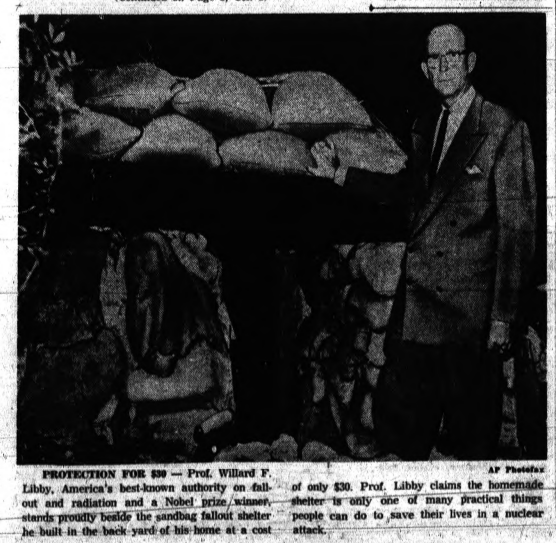
PROTECTION FOR $30 — Prof. Willard F. Libby, America's best-known authority on fallout and radiation and a Nobel prize winner, stands proudly beside the sandbag fallout shelter he built in the back yard of his home at a cost
