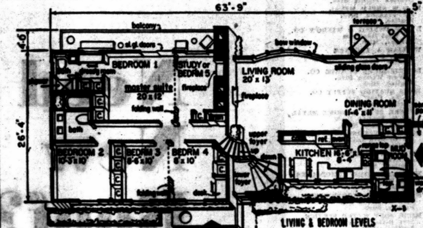
UPPER LEVELS — The bedroom and living room areas of the house are shown in the floor plan above. Depending on the size of the family, there can be three, four or five bedrooms. The living room and dining room are across the back of the house with a terrace outside.
