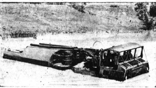
THIS MACHINE 'SWIMS' — Mobility, agility and durability are the features claimed for the "Goer," shown fording a stream. The Army is testing the vehicle to see whether it's capable of transporting military supplies
