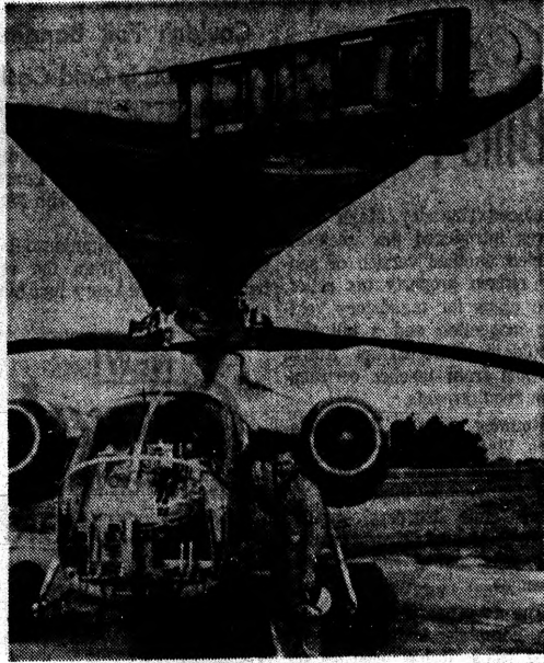
'HOT CYCLE' — Hughes Aircraft yesterday showed newsmen the Army's XV9A "hot cycle" helicopter, which jets high-energy gases from rotor blades like this. The research copter is propelled by ducting gases from a turbojet engine to the rotor tips where they are exhausted. Hughes said the "hot cycle" gets rid of heavy drive shafts used in conventional helicopters.
