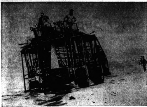
BLUEBERRY PICKER —A mechanical blueberry picker, manufactured in Grand Haven, is tested on beach sand along Lake Michigan. The driver sits 12 feet up and rides on swamp buggy tires at 6 miles an hour. The 11,000-pound vehicle shakes berries
