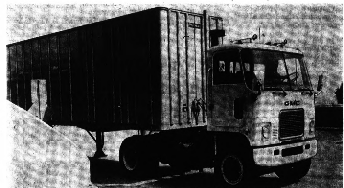
REGULAR CAB STYLE—Among the 1969 models unveiled by GMC Truck & Coach Division today is this heavy-duty Astro 95 model, with a regular (nonsleeper) cab. The 54-inch cab is aluminum and tilts forward to provide 90-degree accessibility.
