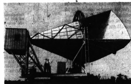
Giant ultra-sensitive horn-reflector antenna which received signals bounced off the satellite. It is located at Bell Telephone Laboratories, Holmdel, New Jersey.
