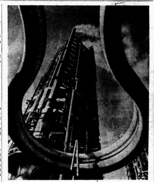
NEW TEXAS GIANT — Steam line expansion loop frames latest Texas skyscraper, a 330-foot tall, 28,000-barrels-per-day catalytic cracking unit, put into operation at Beaumont.
